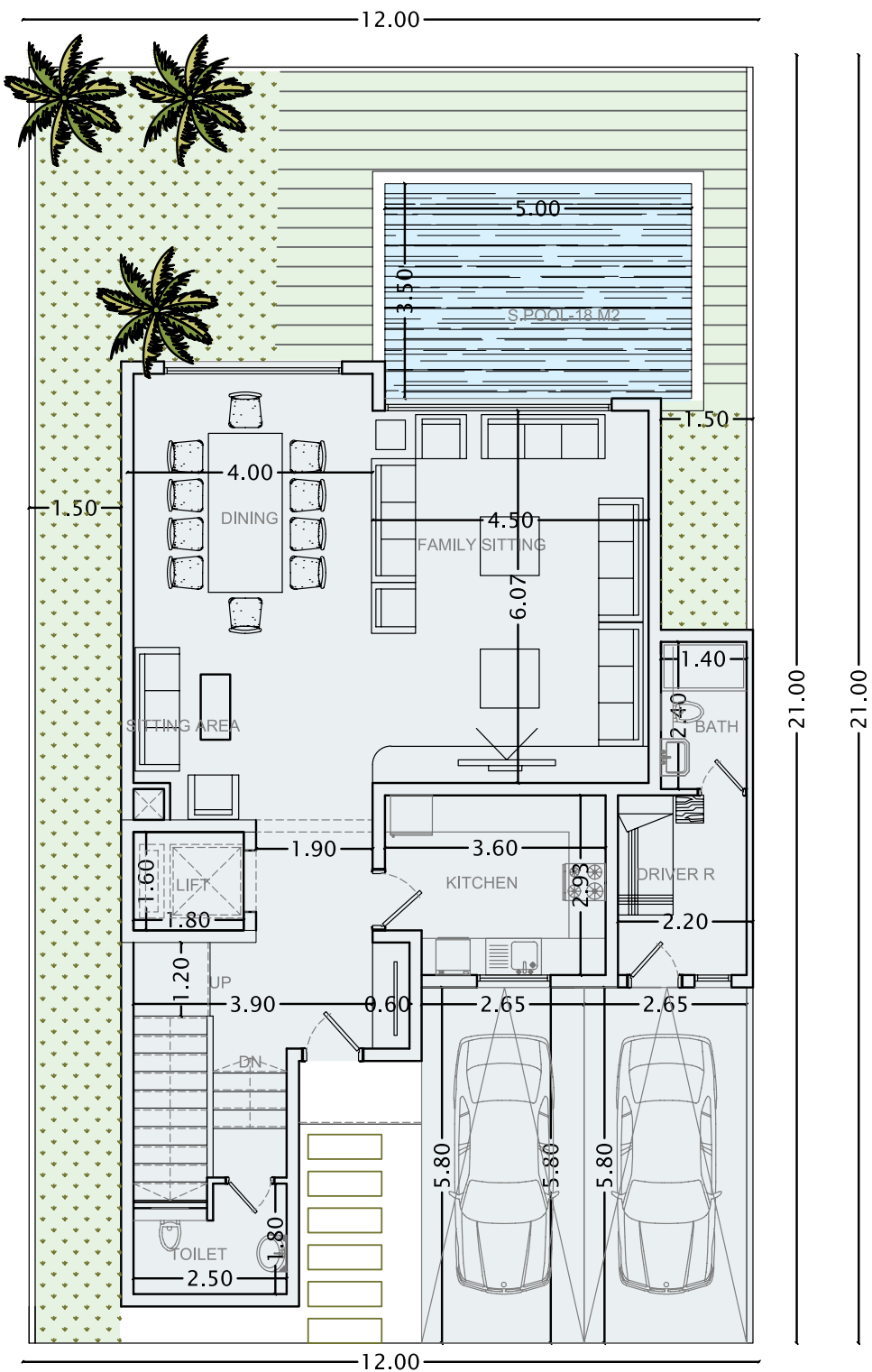
Ground floor
