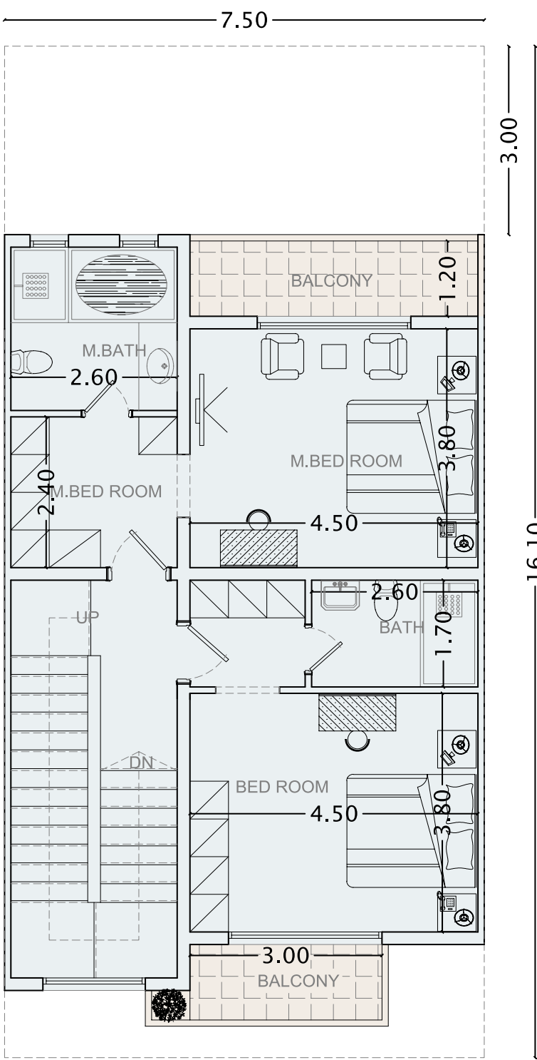
First floor Floor Area=80.88 sqm Balcony=10.4 sqm Total BUA= 91.28 sqm
