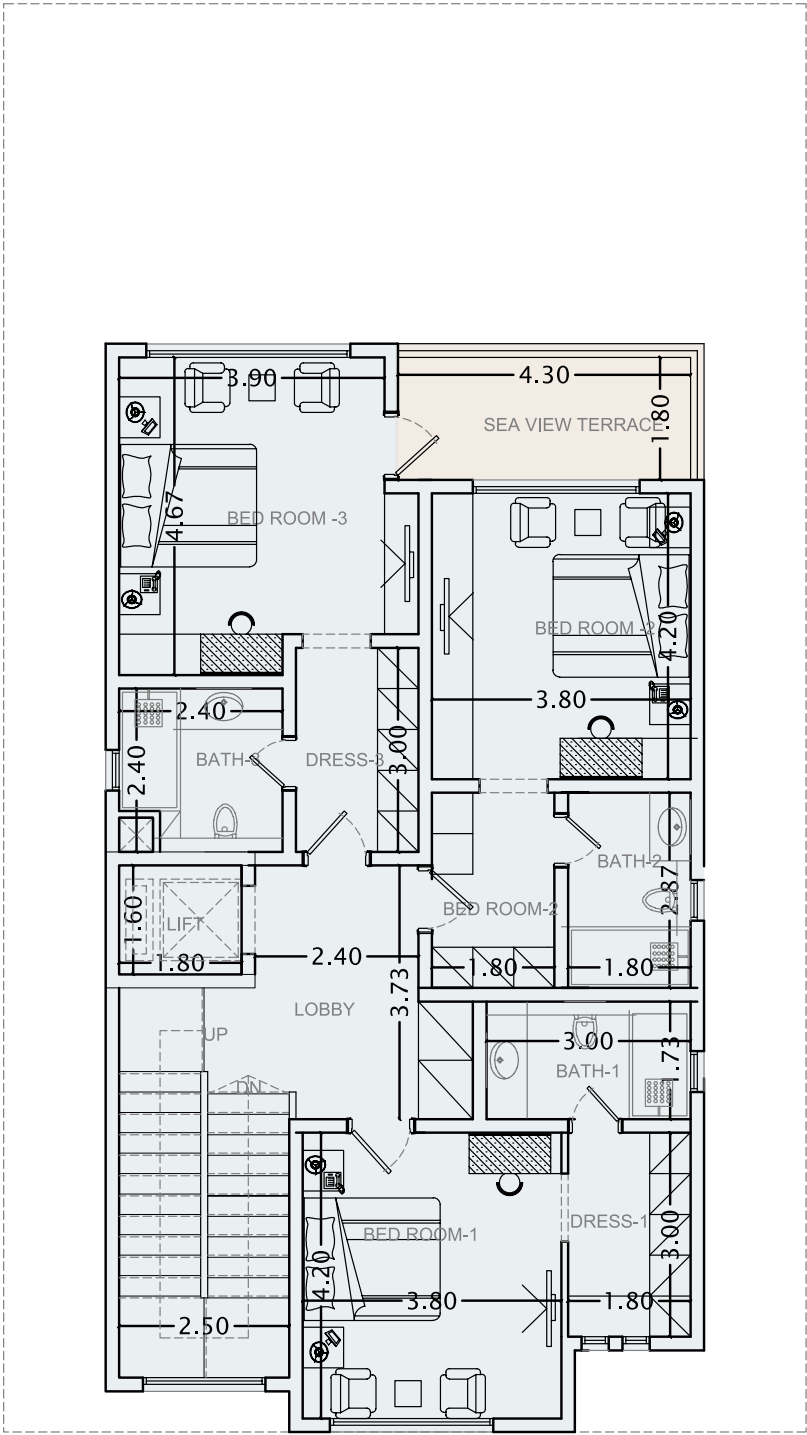
First floor
