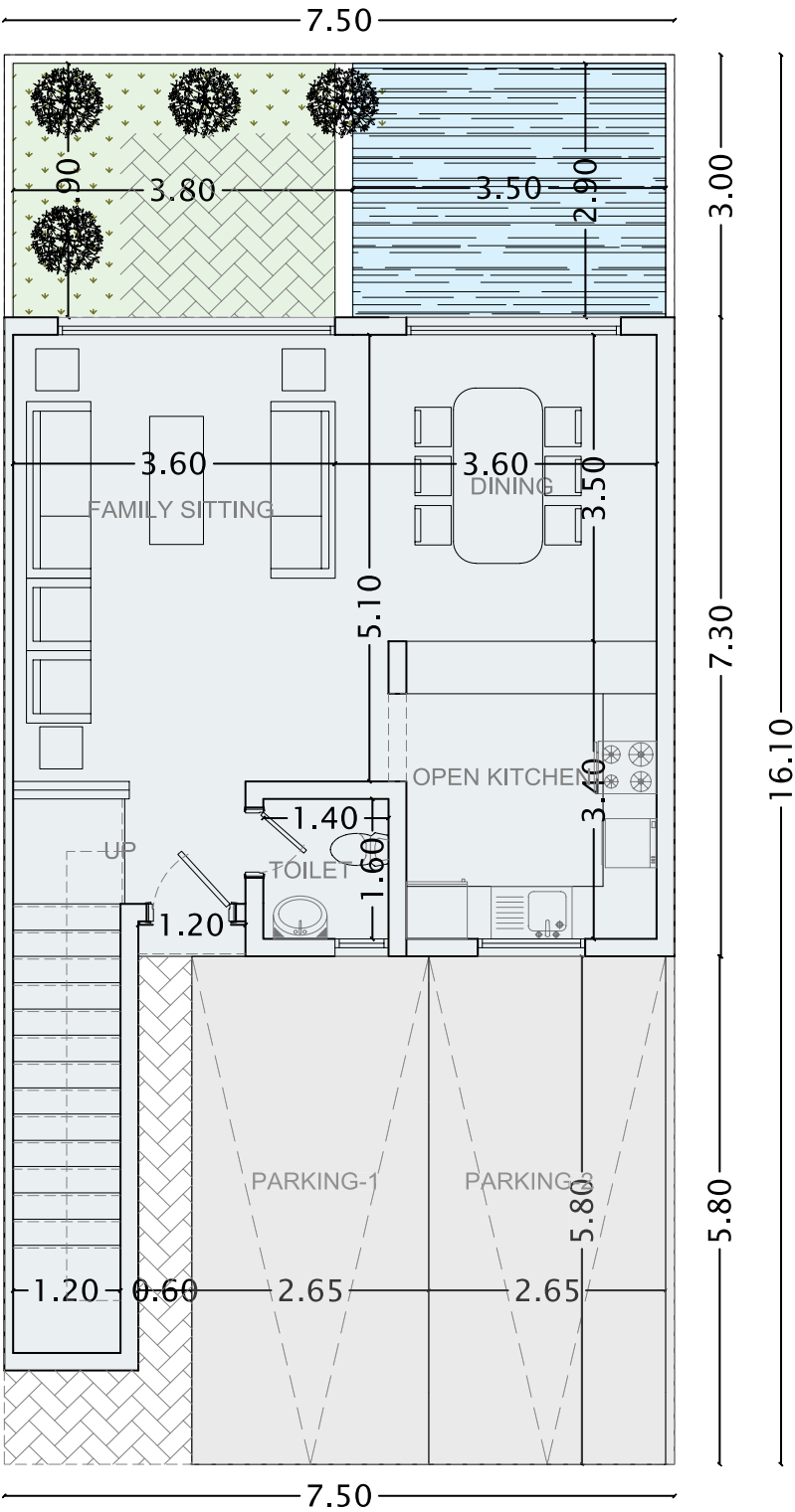
Ground floor Floor Area=61.84 sqm Garden=29.22 sqm Parking=31.30 sqm Total BUA= 93.14 sqm
