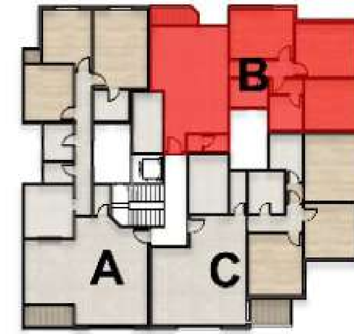
BUILDING 1&11 TYPICAL
