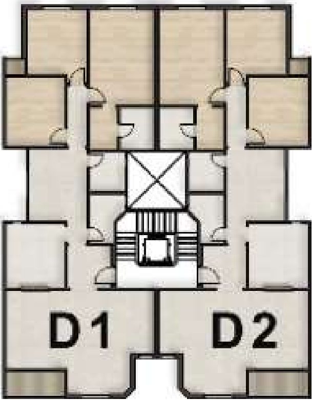
BUILDING 2 TO 10 TYPICAL
