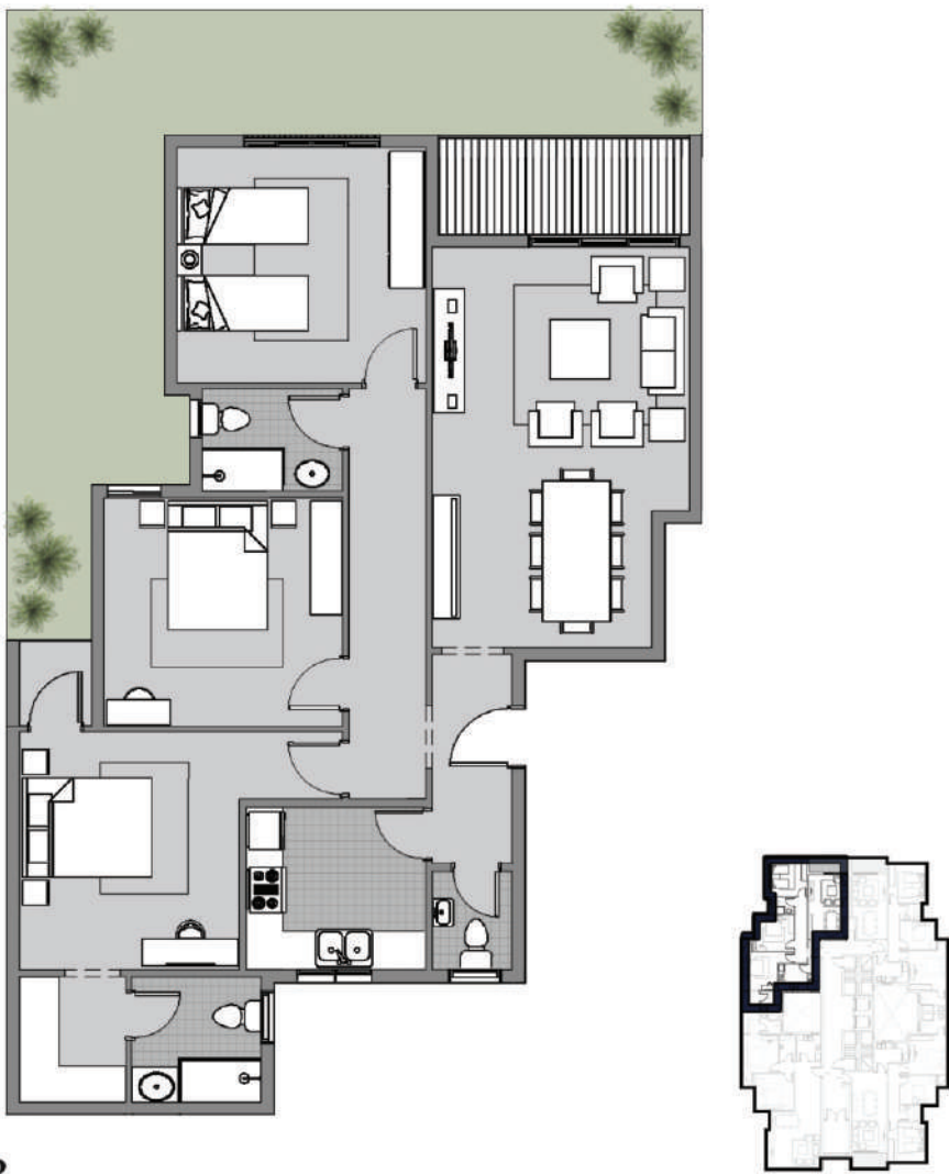
Dejoya 4 Type -A Ground Floor Plan GROSS AREA= 165 SQ.METER
