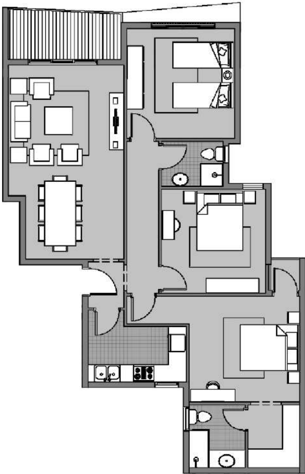
Dejoya 4 Type -B Second Floor Plan GROSS AREA= 156 SQ.METER
