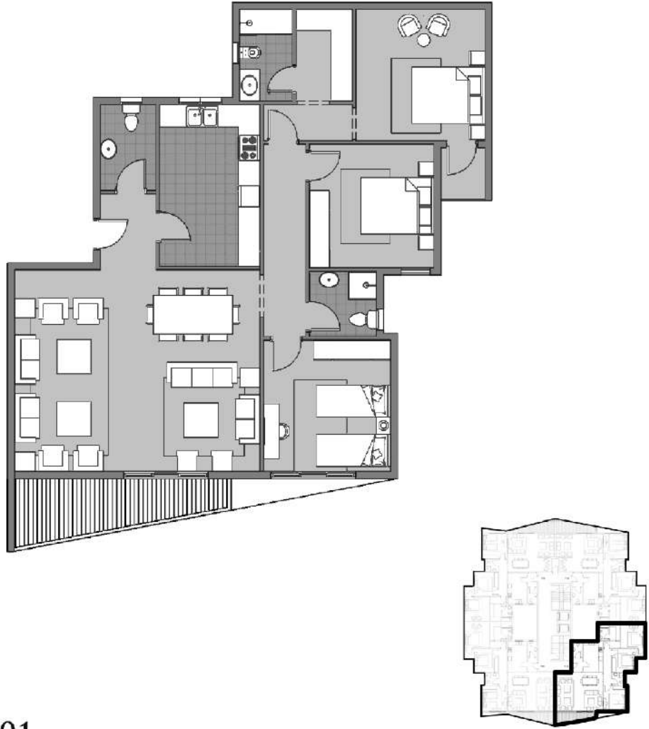
Dejoya 4 Type -C First Floor Plan GROSS AREA= 193 SQ.METER
