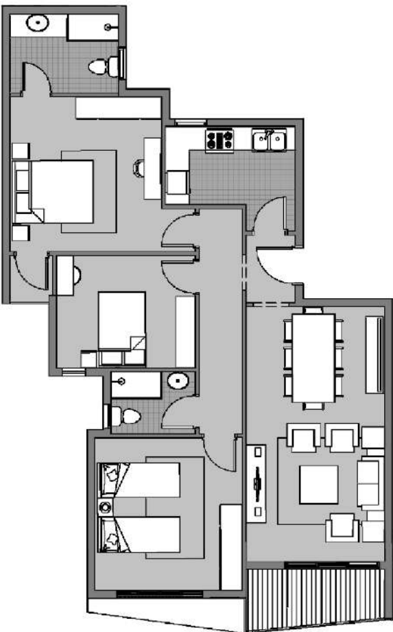
Dejoya 4 Type -B Third Floor Plan GROSS AREA= 143 SQ.METER
