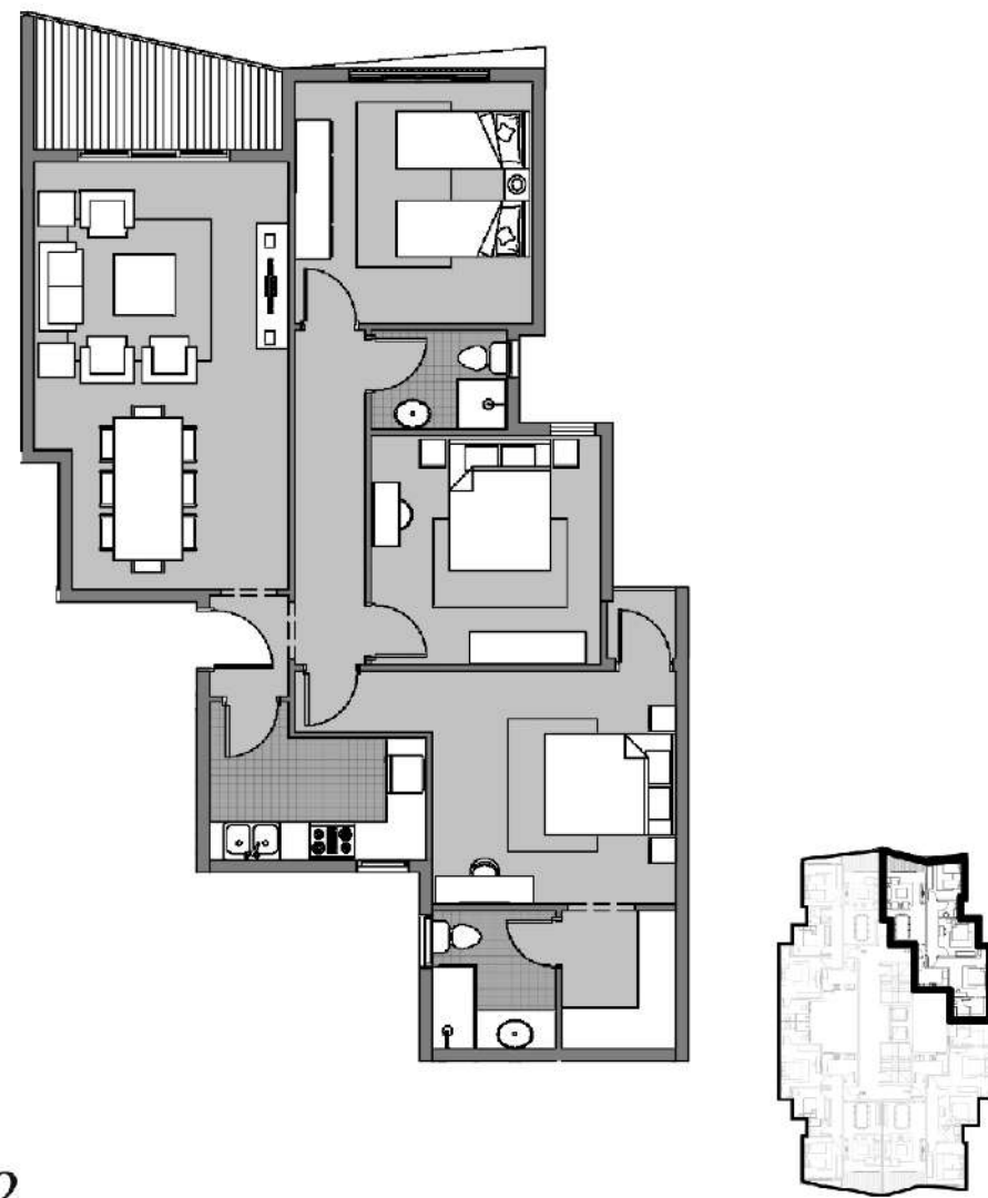
Dejoya 4 Type -B Fourth Floor Plan GROSS AREA= 156 SQ.METER
