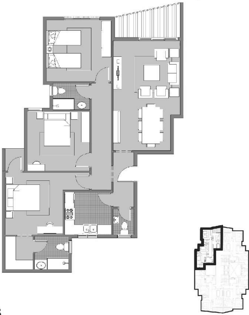
Dejoya 4 Type -A First Floor Plan GROSS AREA= 167 SQ.METER
