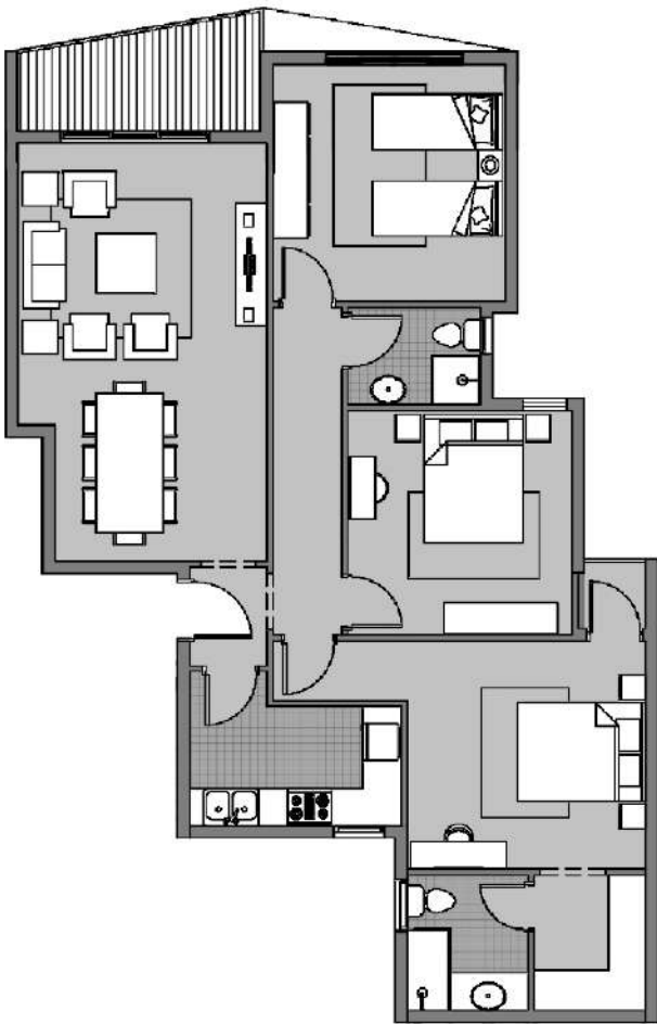
Dejoya 4 Type -B Third Floor Plan GROSS AREA= 155 SQ.METER
