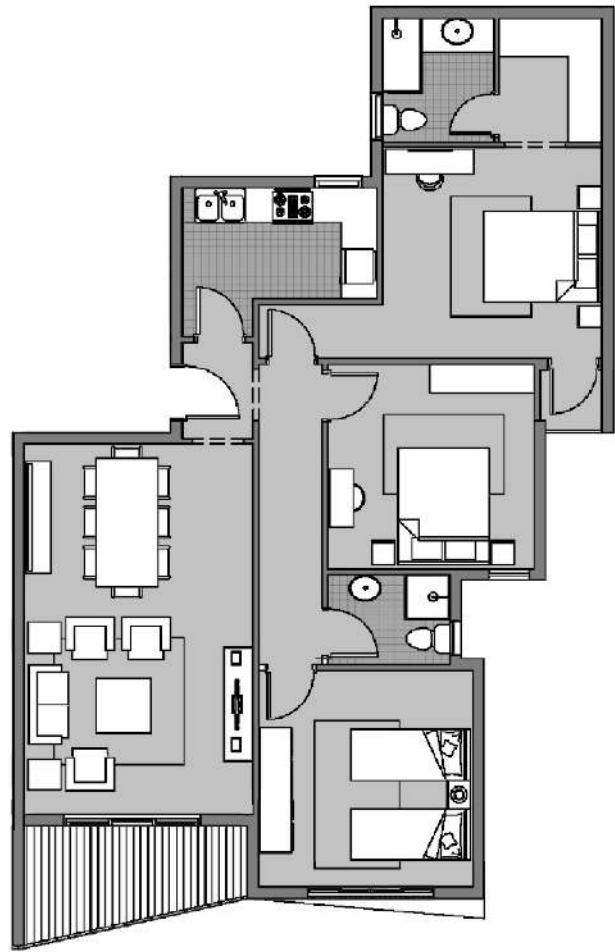
Dejoya 4 Type -B FIRST Floor Plan GROSS AREA= 157 SQ.METER
