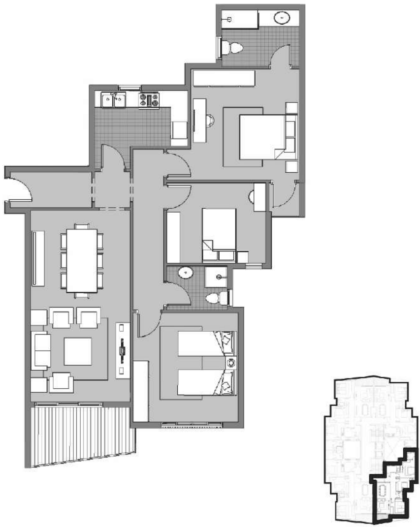
Dejoya 4 Type -A First Floor Plan GROSS AREA= 152 SQ.METER
