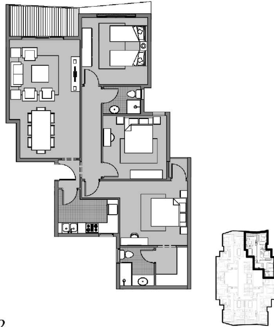
Dejoya 4 Type -B Fifth Floor Plan GROSS AREA= 156 SQ.METER
