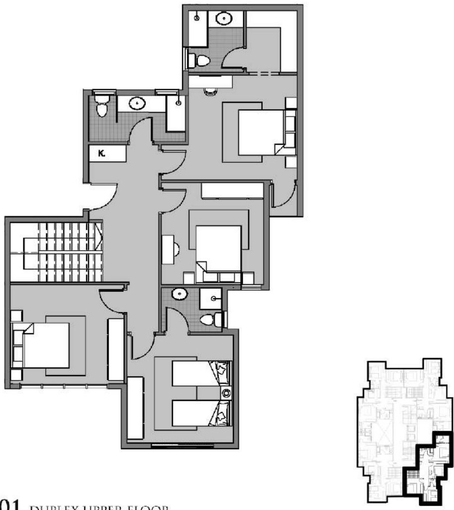
UNIT-D01 DUPLEX UPPER FLOOR
