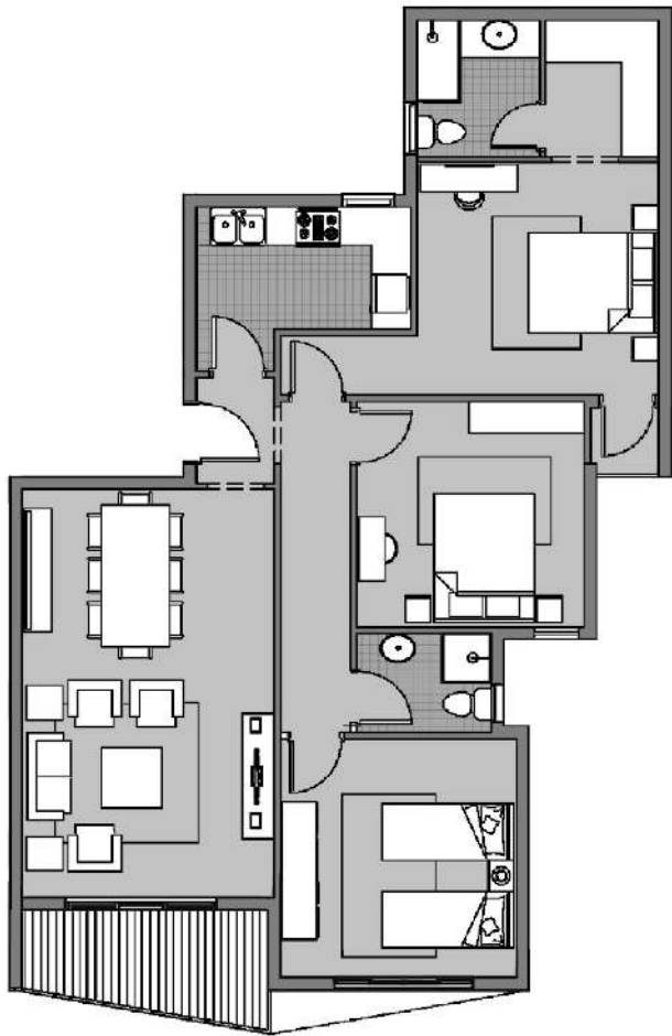
Dejoya 4 Type -B Third Floor Plan GROSS AREA= 156 SQ.METER
