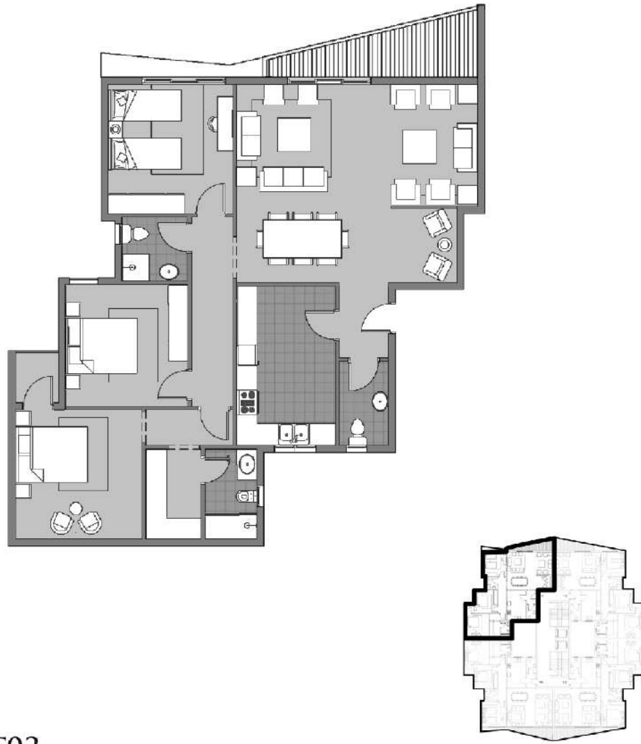
Dejoya 4 Type -C First Floor Plan GROSS AREA= 189 SQ.METER
