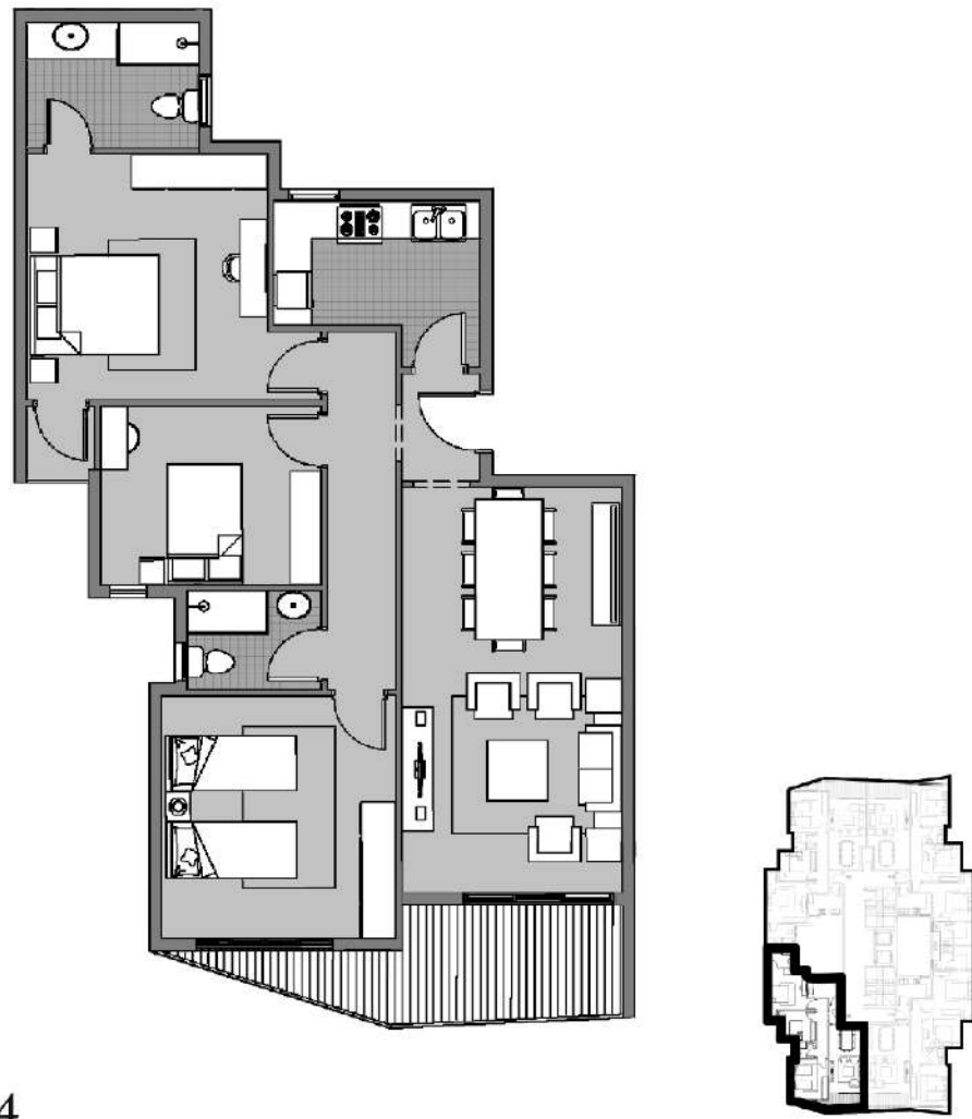
Dejoya 4 Type -B Fifth Floor Plan GROSS AREA= 149 SQ.METER
