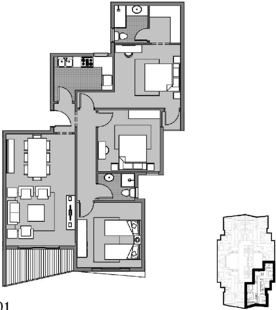
Dejoya 4 Type -B Fourth Floor Plan GROSS AREA= 157 SQ.METER
