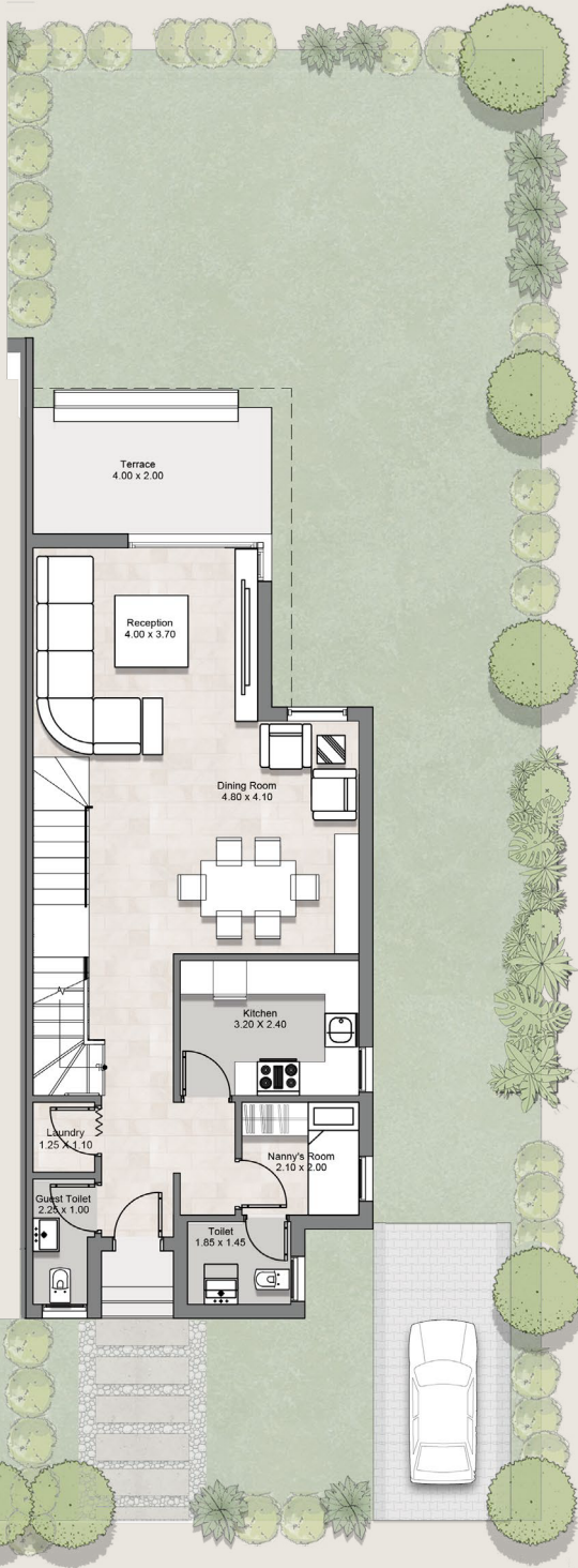
GROUND FLOOR
