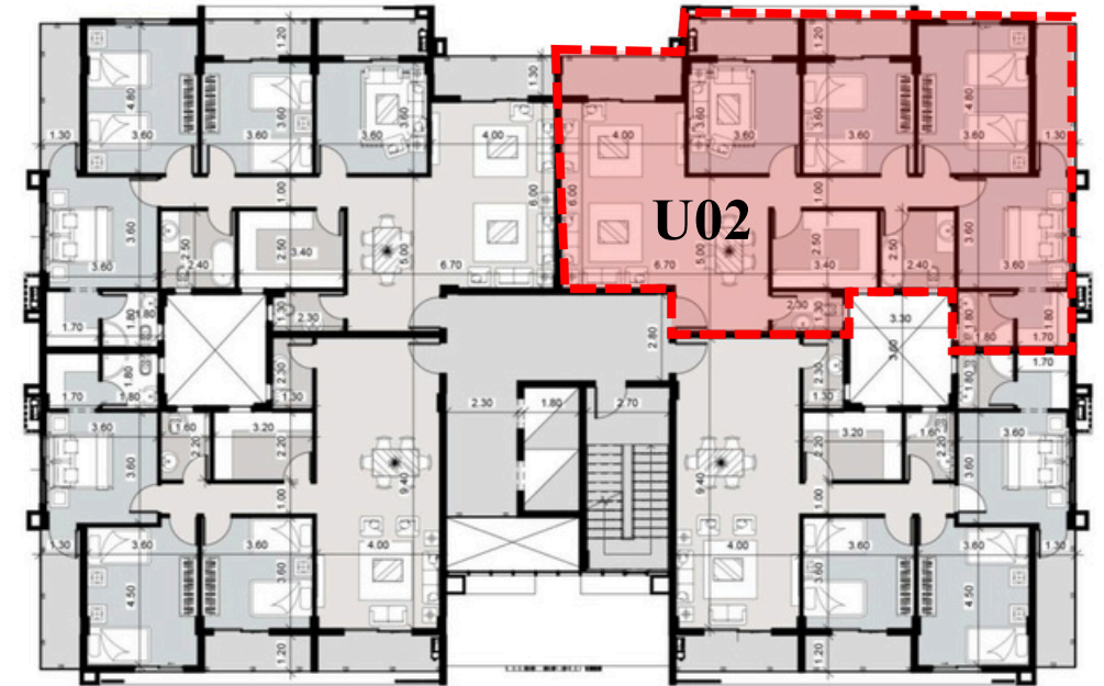
TYPE (B) FIRST FLOOR
