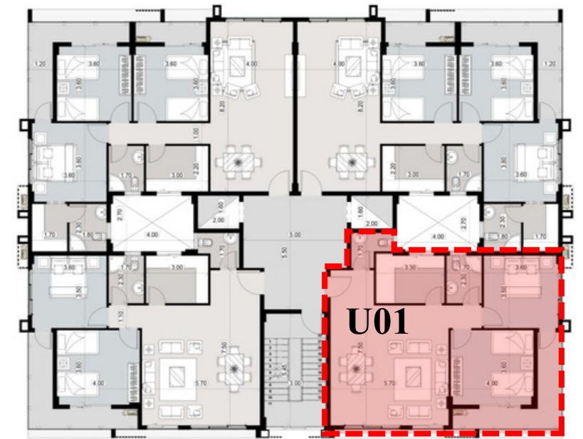
TYPE (C) SECOND FLOOR
