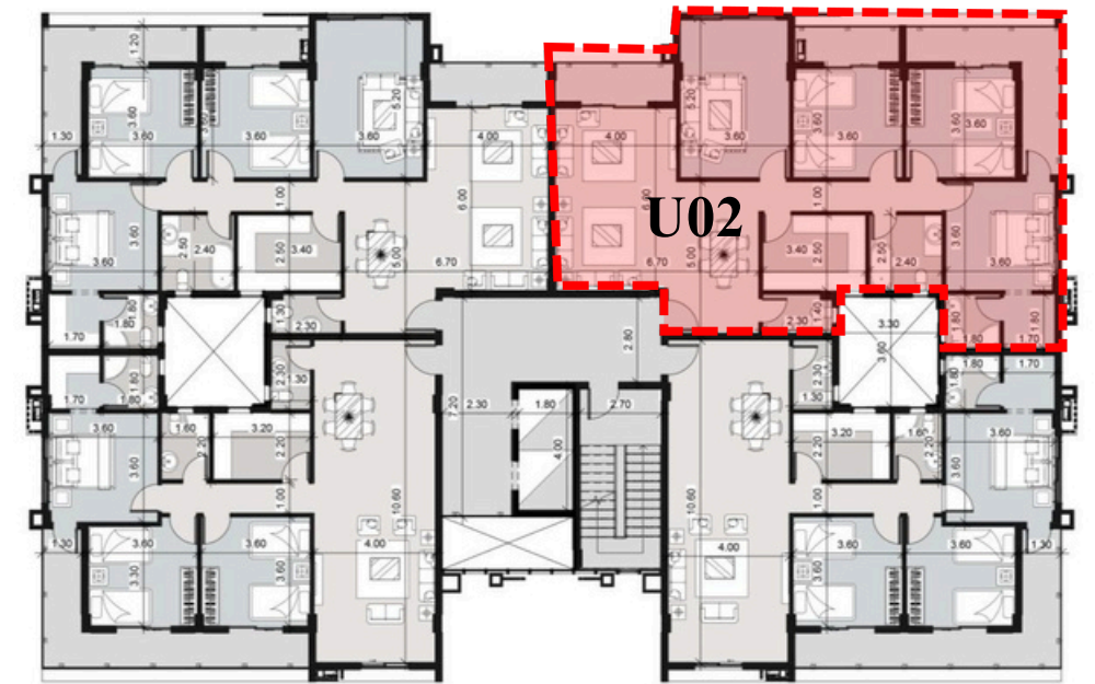
TYPE (B) SECOND FLOOR
