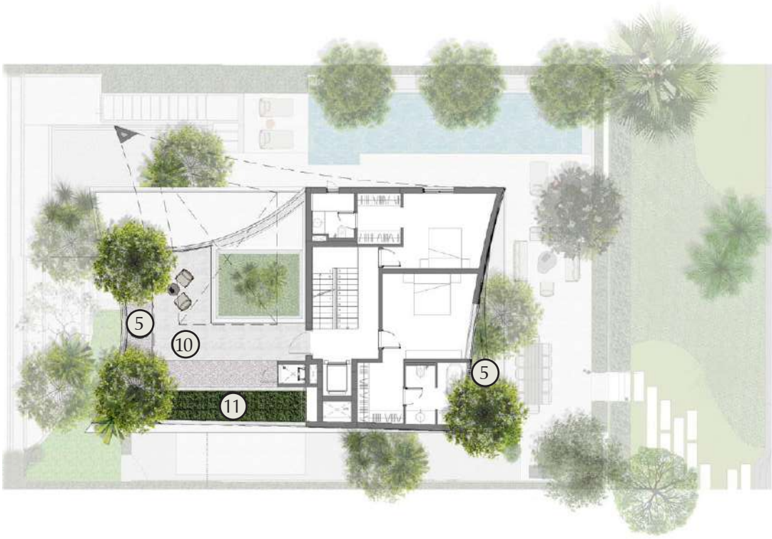
ROOF FLOOR
