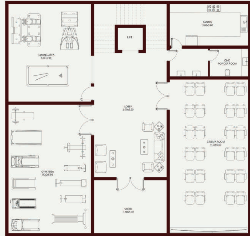
BASEMENT
