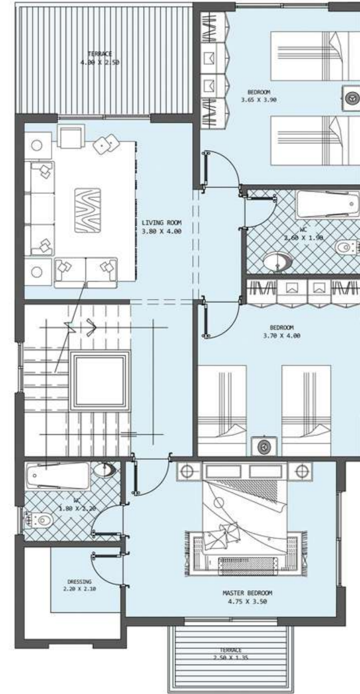
FIRST FLOOR 151.56
